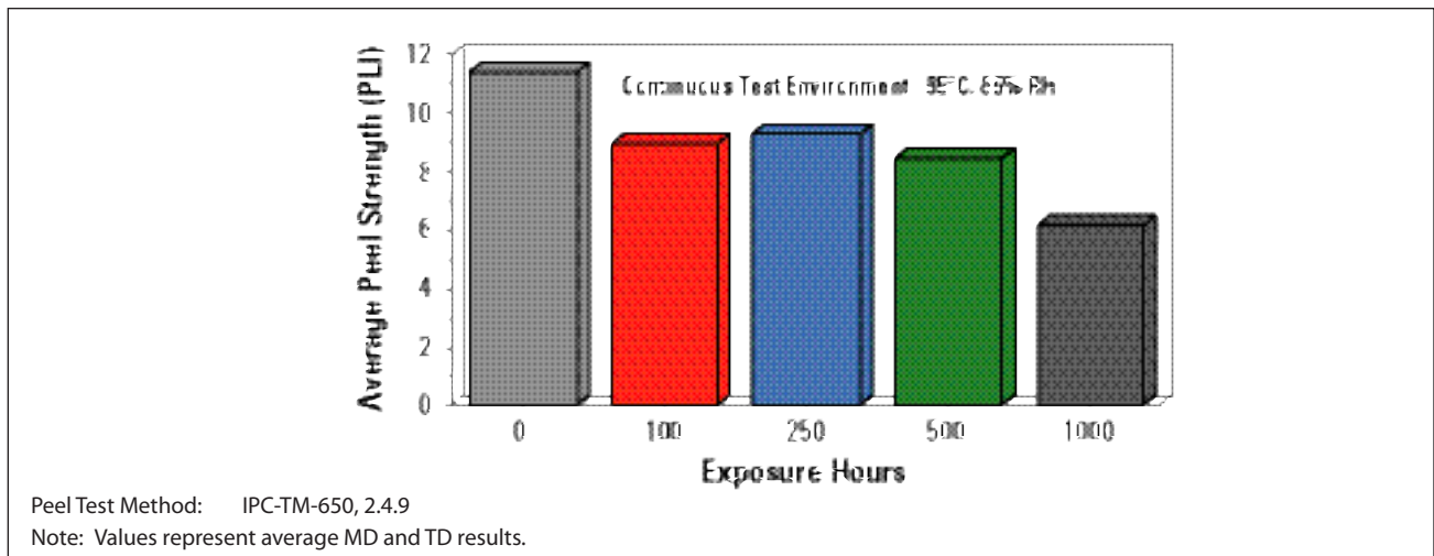
Figure 5. Temperature/Humidity Exposure
